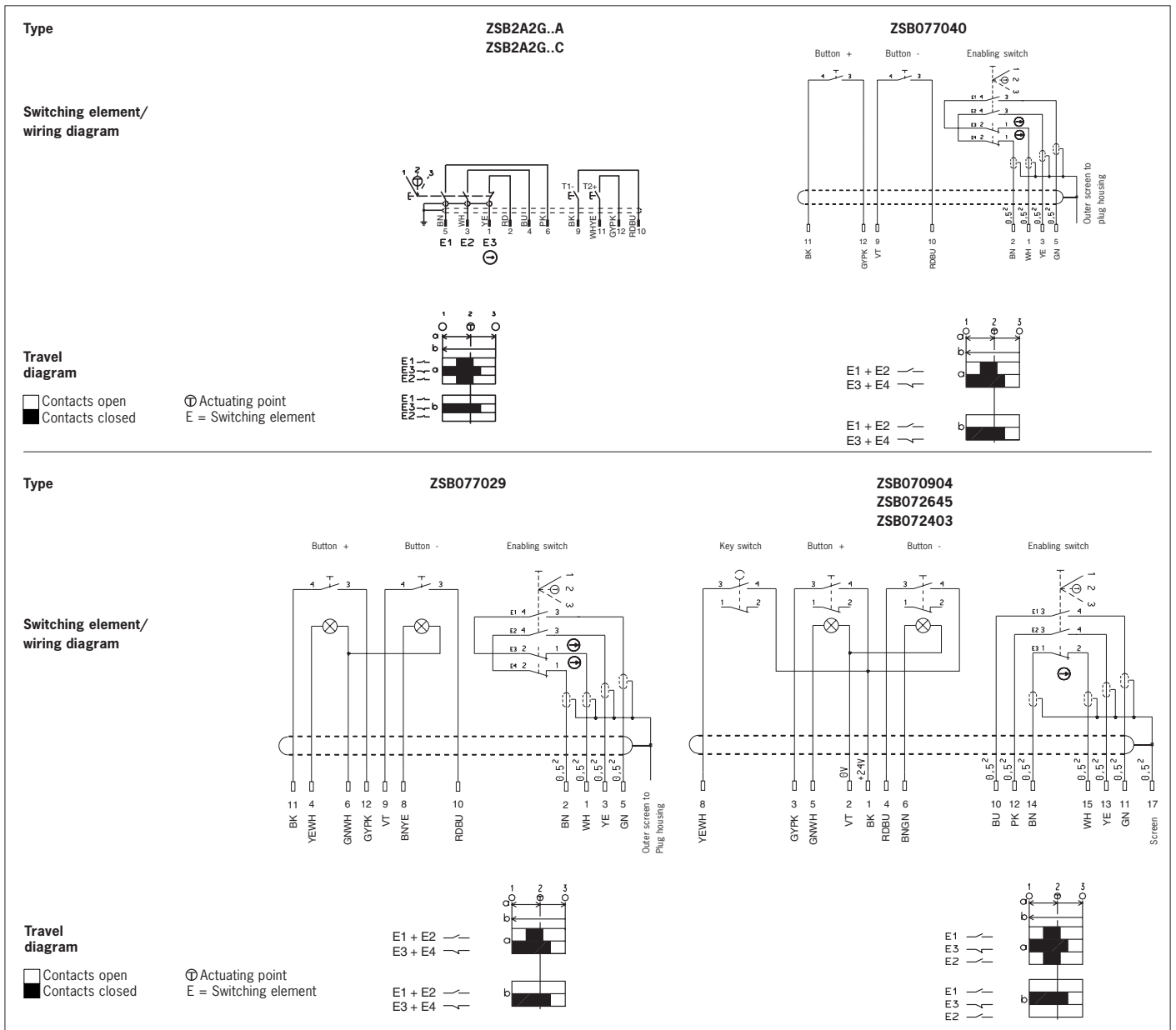
Figure 1: Function of the switching elements and wiring diagrams
