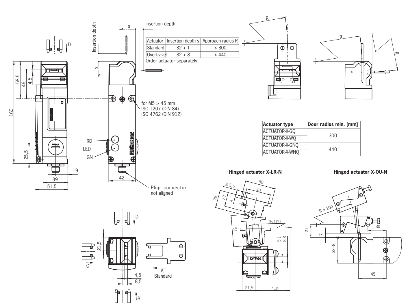
Figure 4: Dimension drawing NX...AS1, insertion depth and approach radii
