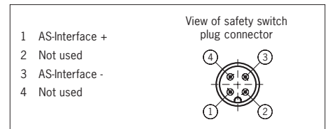
Fig. 3: AS-Interface M12 plug connector terminal assignment
