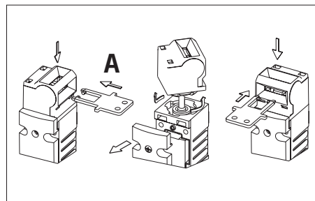
Fig. 1: Changing the actuating direction
