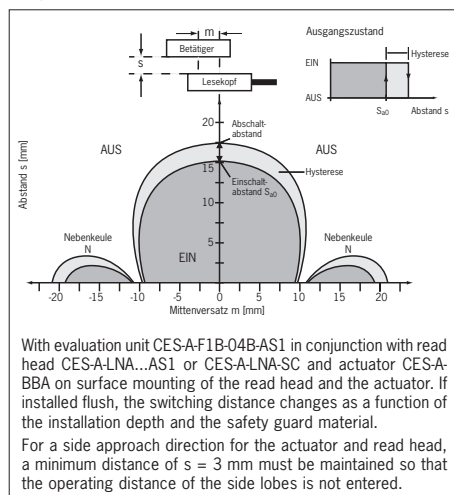
Fig. 3: Typical operating distance
