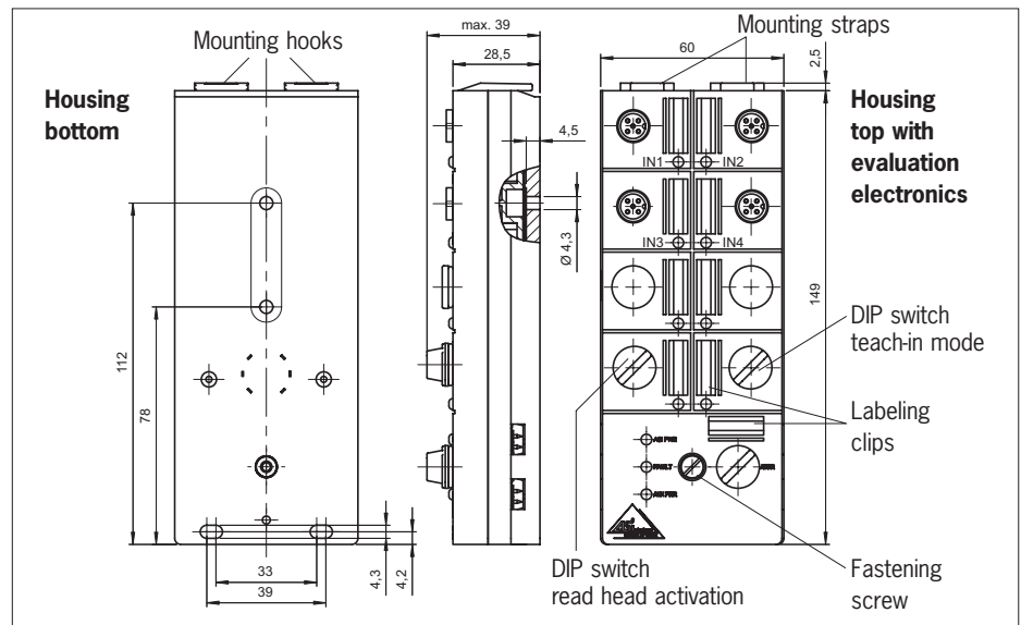
Figure 2: Dimension drawing CES...AS1 (Illustration shows version CES-A-F1B-04B-AS1)
